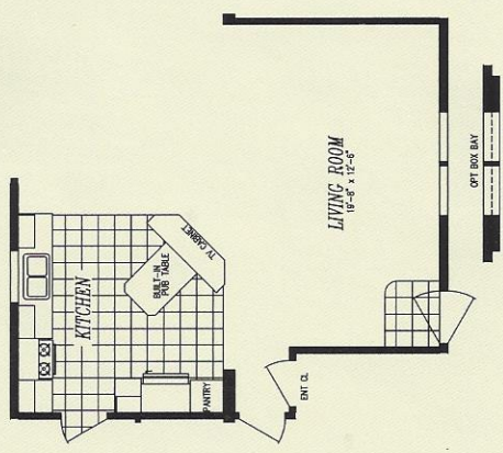
ALTERNATE KITCHEN DESIGN WITH BUILT-IN PUB TABLE
