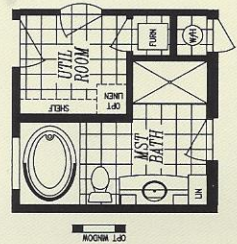
DELUXE BATH OPTION WITH 60" SHOWER
