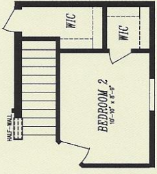
HUD STAIRWELL OPTION
