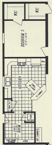
ALTERNATE KITCHEN DESIGN WITH BUILT-IN PUB TABLE
